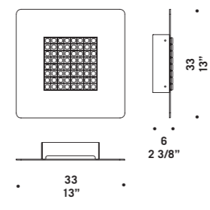
ROMA A/P 33 25W 2700lm LED 2700K CRI90 CE IP20 □
