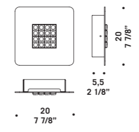
ROMA A/P 20 9W 900lm LED 2700K CRI90 CE IP20 □
