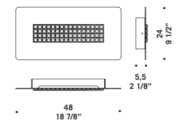
ROMA A/P 48-24 25W 2700lm LED 2700K CRI90 CE IP20 □
