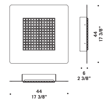
ROMA A/P 44 38W 4000lm LED 2700K CRI90 CE IP20 □
