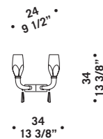
FLUTE A2 2 x max 33W G9 HSGST/C/UB alogeno bispina halogen bi-pin 2 x G9 LED LED light bulb
